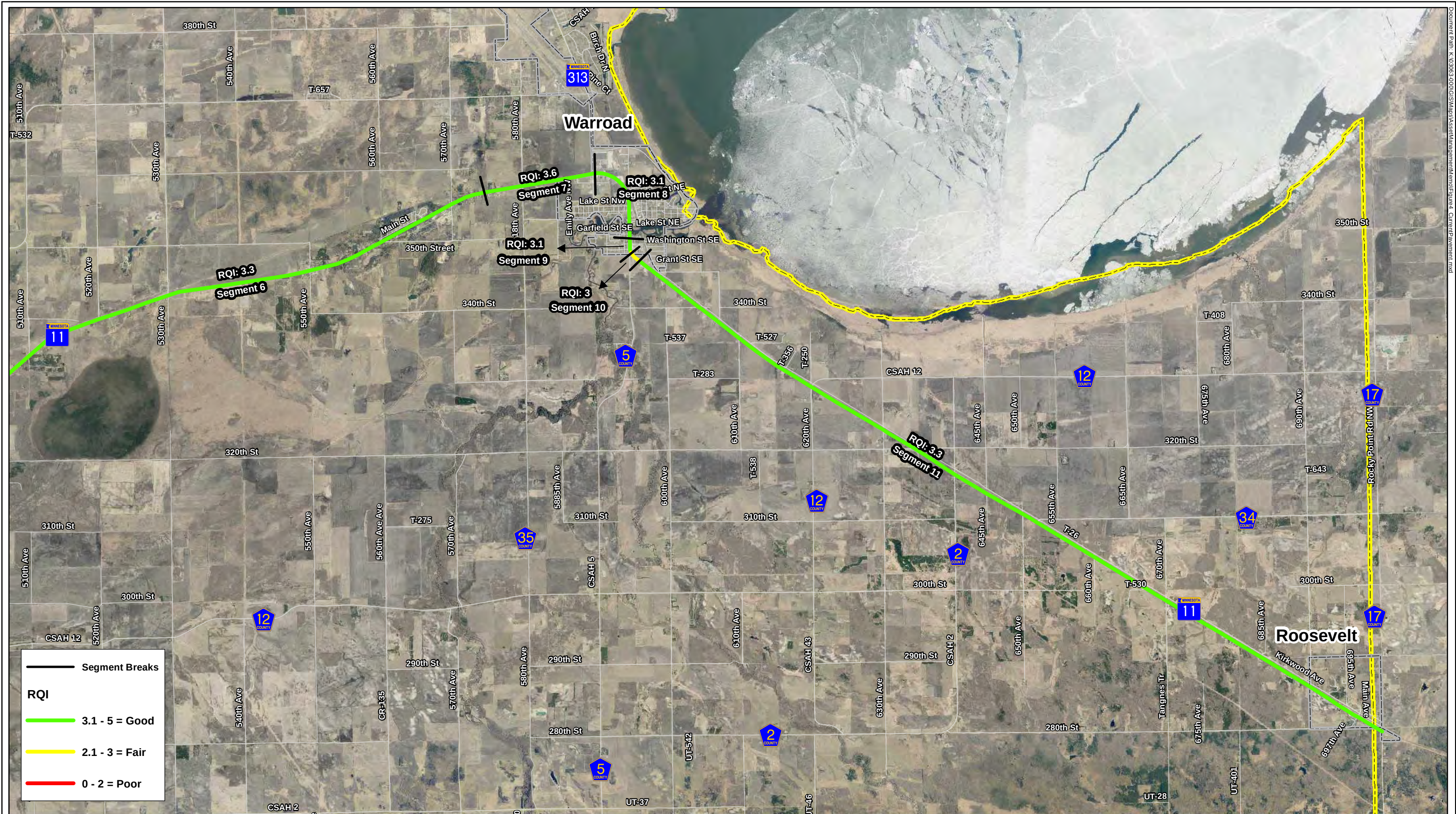
Figure 4 2014 Pavement Condition Warroad
