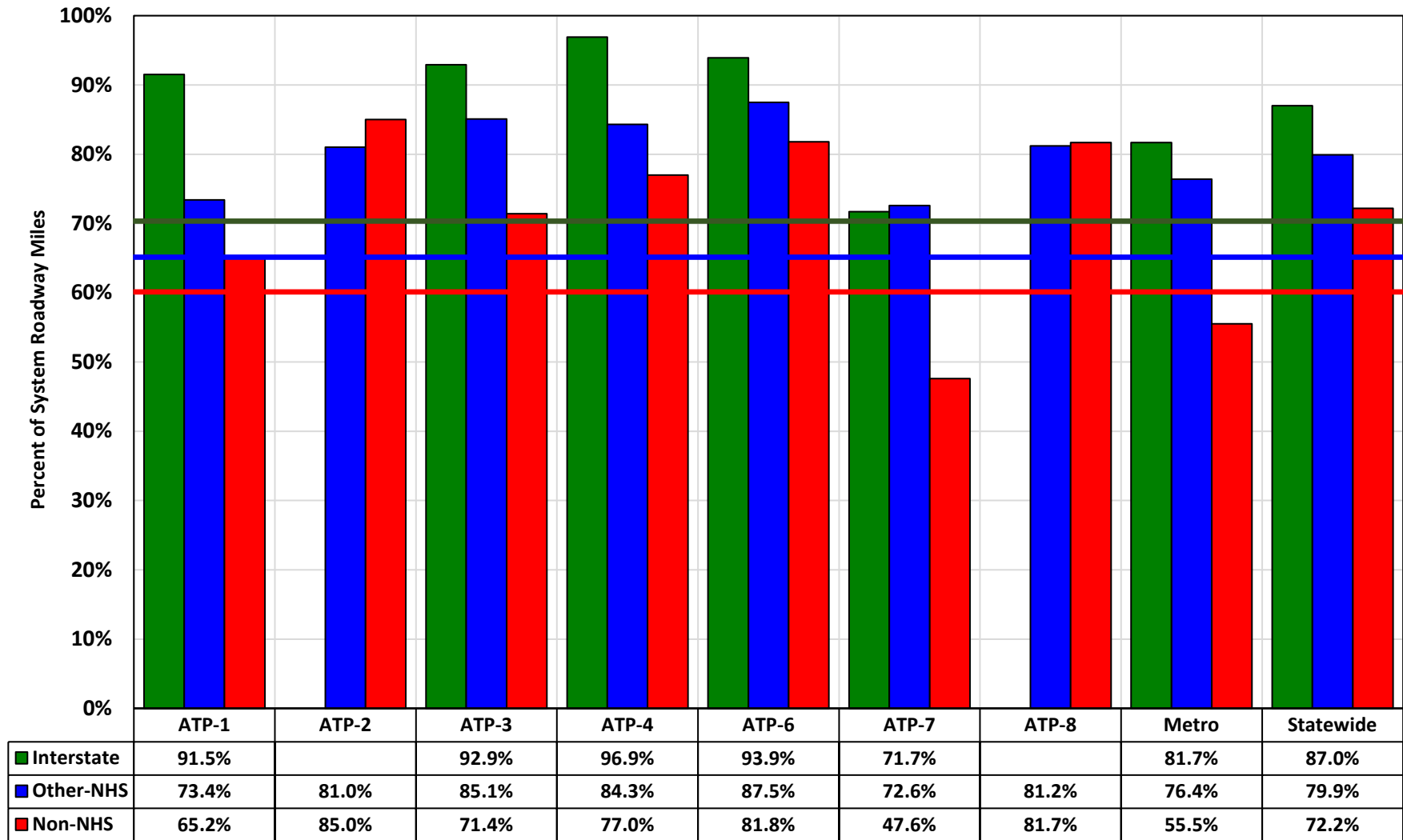
Figure 4 "Good" Ride Quality Index (percent of roadway miles with an RQI greater than 3.0) Comparison of 2020 Data by ATP
