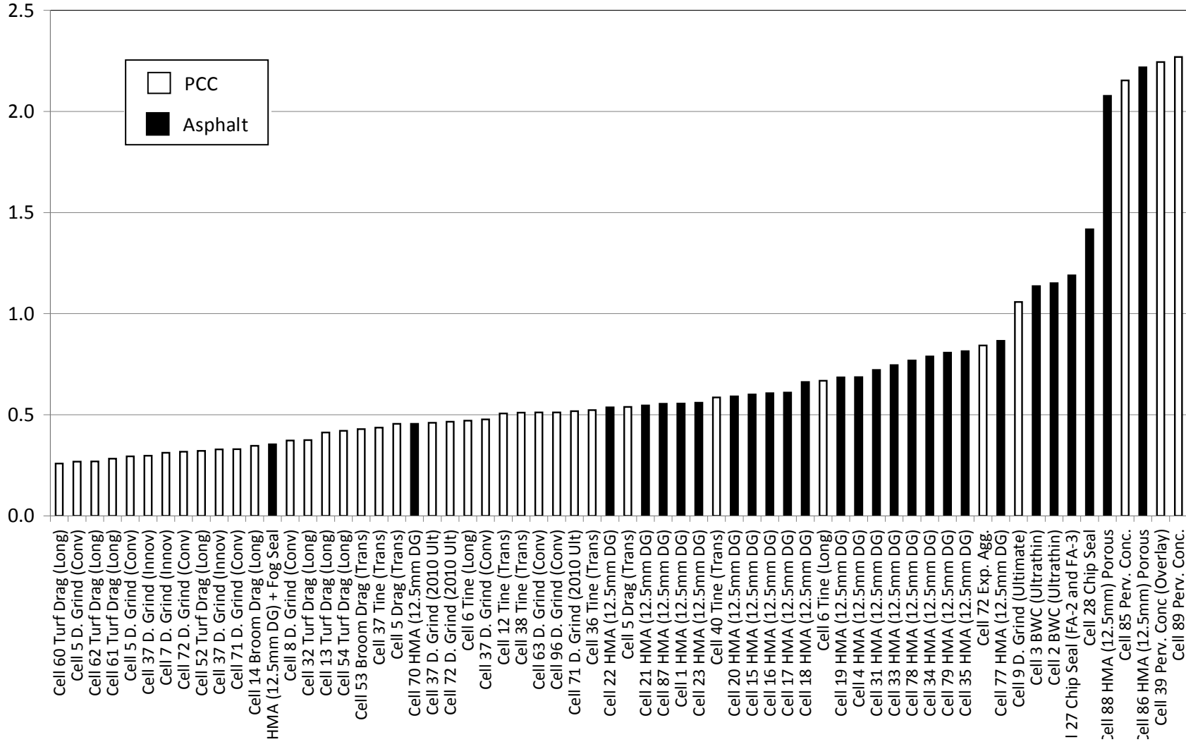
Figure 5-1. Average longitudinal MPD (mm) for all the cells.
